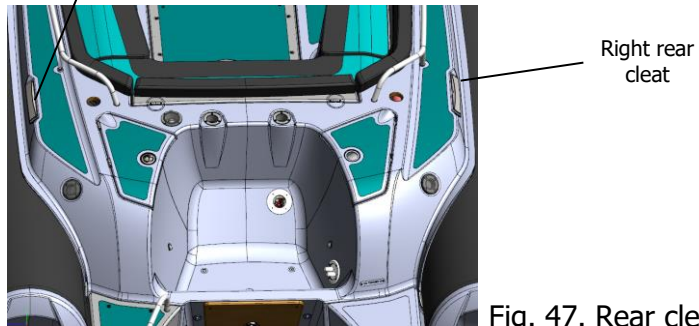
Fig. 47. Rear cleats.
