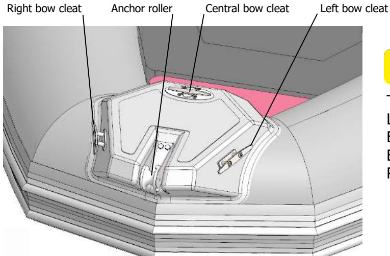
Fig. 61. Bow cleats.
