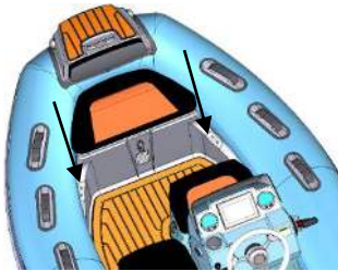
Fig. 29. Bow lifting eyes, 2 positions.
