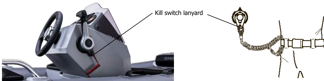
Fig. 22. Engine kill switch lanyard.
